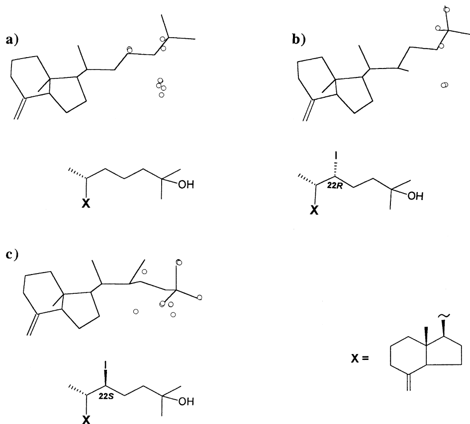
Figure 2. Stereoplot of the global energy minimum conformations (wireframe drawings) of the model 8-methylene compound 14a with 25-hydroxyvitamin D 3 side chain (a), its 22 R -iodo substituted analogue 14b (b), and isomeric compound 14c (c). The circles show the location of 25-oxygen atoms in the other higher energy conformers (energy window 1 kcal/mol). All hydrogen atoms are omitted.
