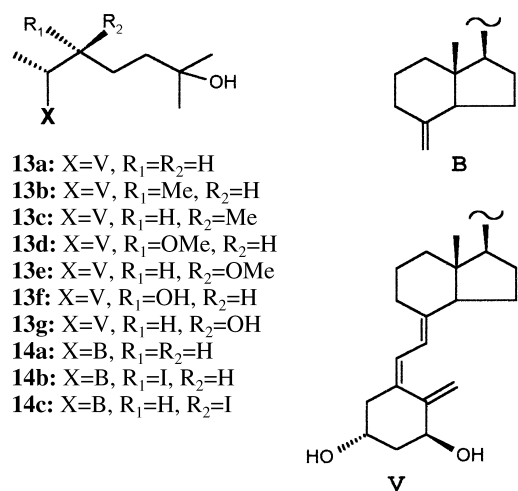
Figure 1. Chemical structure of 1 \alpha ,25-dihydroxyvitamin D 3 (calcitriol) and its 22-substituted analogues.
