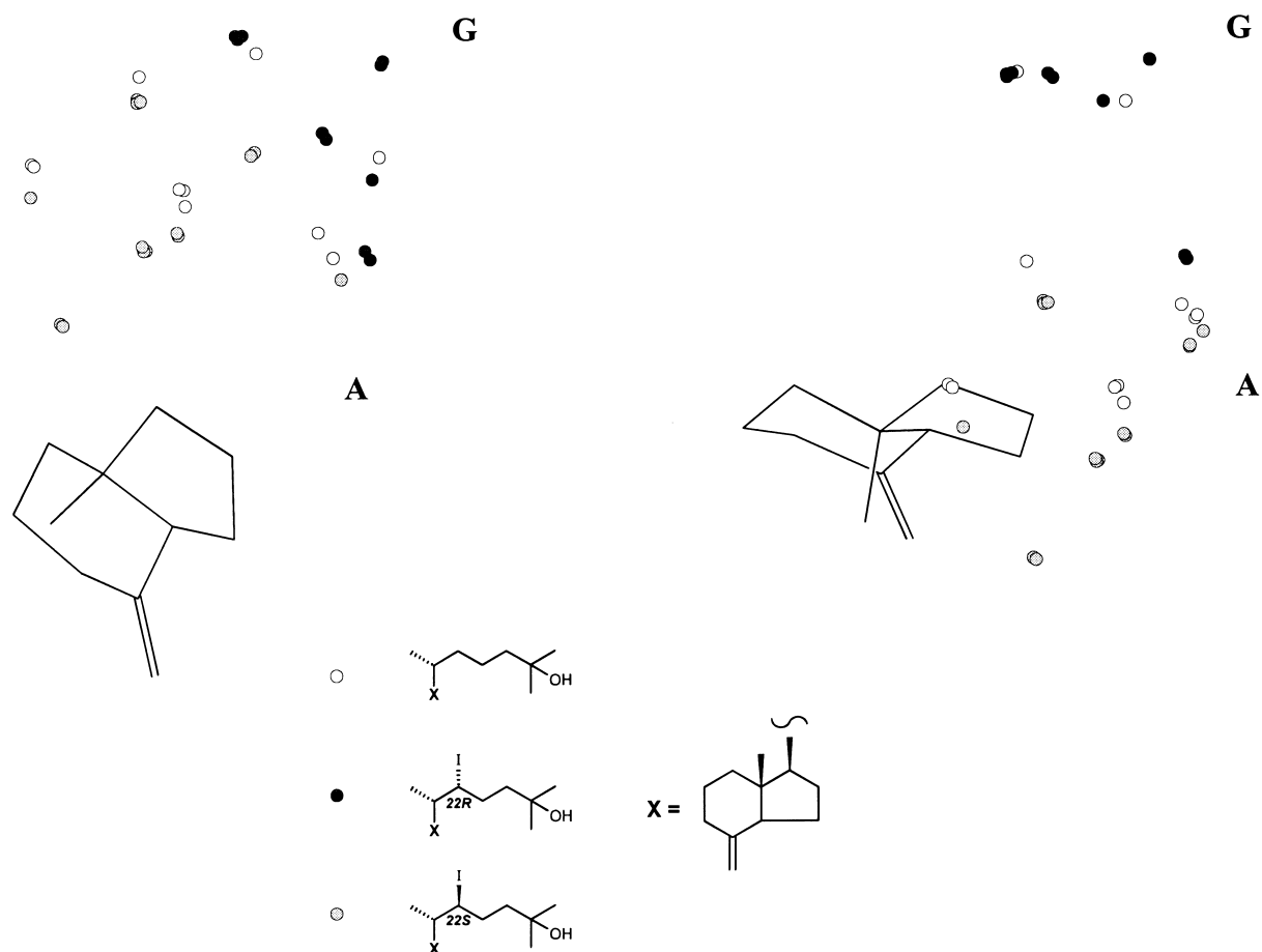
Figure 3. Two different stereoviews illustrating results of conformational analysis of the side chain of model CD-ring compounds 14a–c . Energy-minimized conformations of these compounds (energy window 1 kcal/mol) were overlaid on the global minimum conformer of 14a as described in Experimental. The circles show the location of 25-oxygen atoms in the corresponding conformers. They are indicated two distinct spatial regions A and G defined by Yamada. 39 Side-chain carbons and all hydrogen atoms are omitted for clarity.
